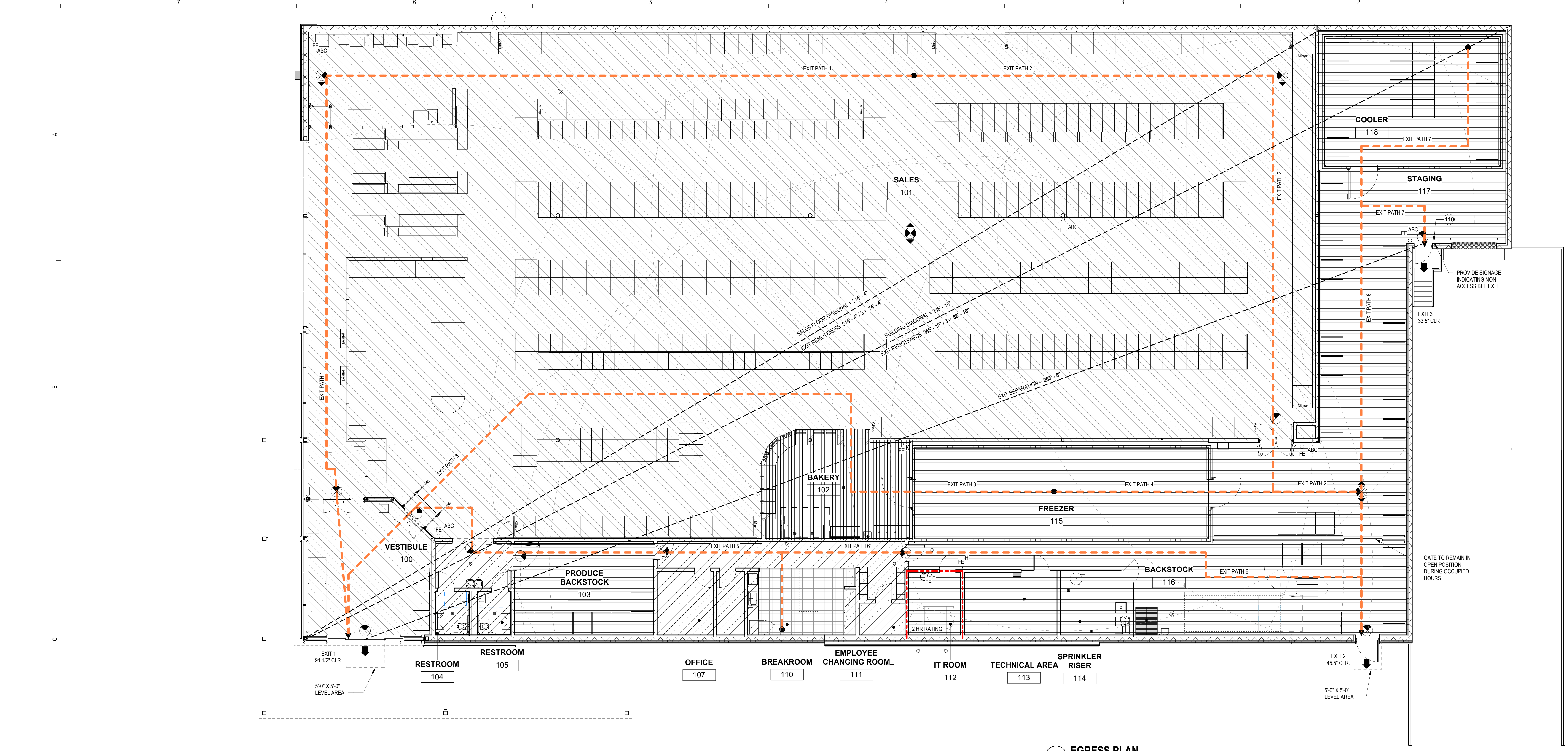
EGRESS PLAN 1/8" = 1'-0"
