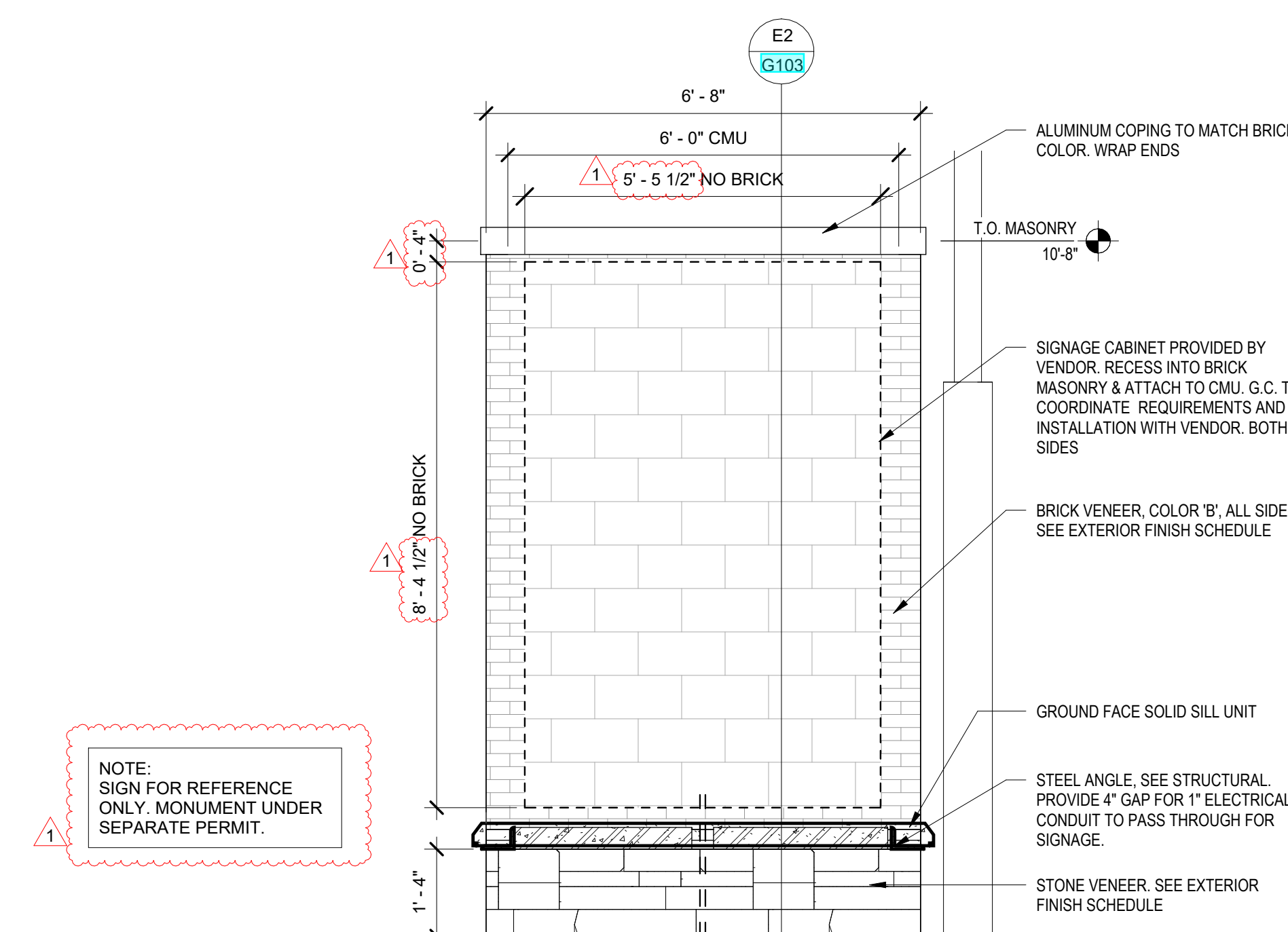
C3 MONUMENT MS-3A ELEVATION 1/2" = 1'-0"
